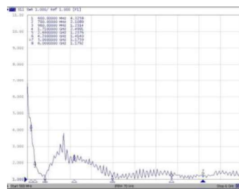
Typical VSWR (Ant1)
