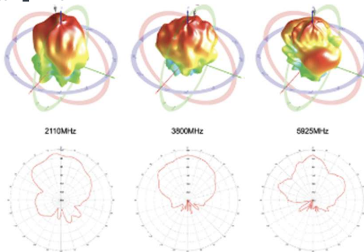
Radiation Pattern_ANT4
